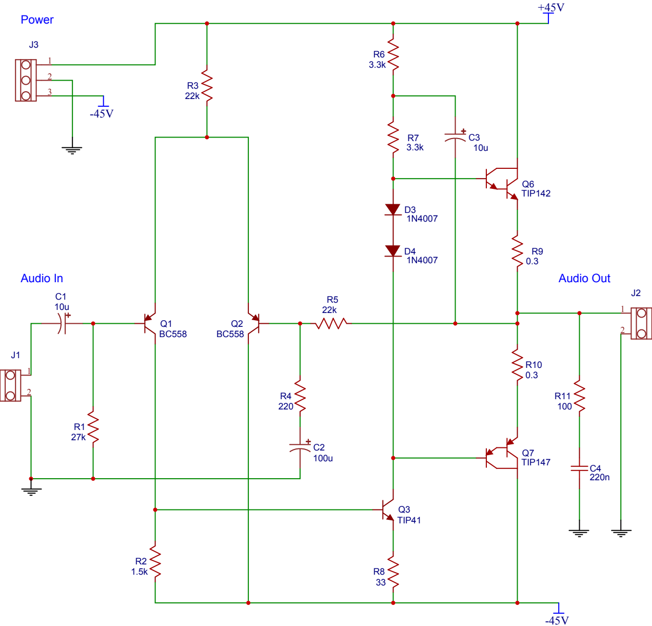
150 Watt audio power amplifier
